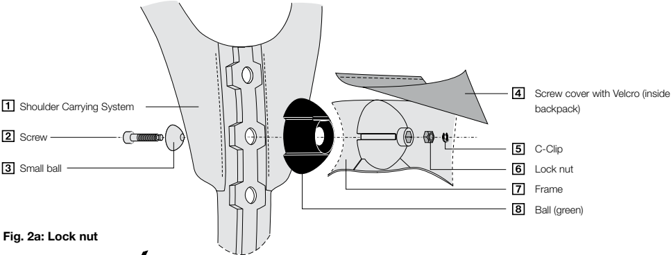
Fig. 2: Ball joint assembly
